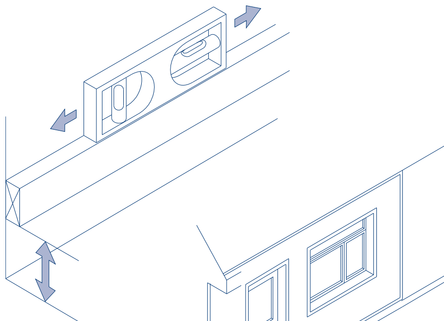
Fig. 1 Check height, line and level of starter batten
