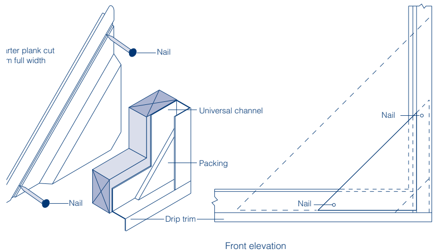
Fig.34 Diagonal plank starter piece Metric view
