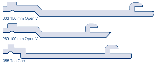
ig.30 Profiles suitable for vertical cladding
