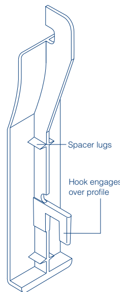
Fig. 22 Rear view of joint cover
