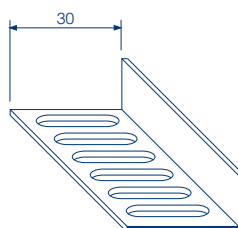
C061 (10 mm type) 30 x 15 mm Angle ventilator
