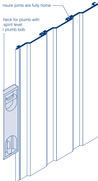
ig.31 Check for plumb every two planks
